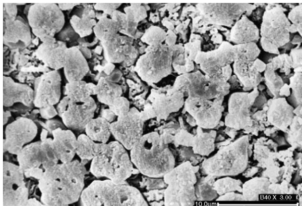
Fig. 6. SEM microstructure of B-CM15Z2.5 glass ceramic glaze.
